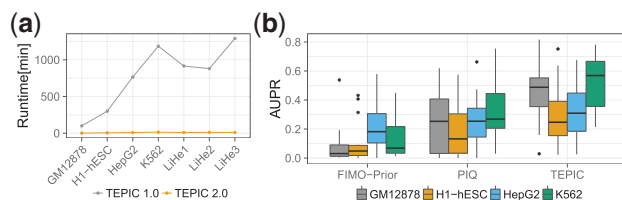
Fig. 1. (a) Runtime comparison of TEPIC to TEPIC 2 using a subset of 458 human TFs. While the original implementation ran up to 1300 minutes to compute TFBS, TEPIC 2 is able to compute TF affinities for peaks in the vicinity of genes in at most 15 minutes. We used four cell line samples and three primary human hepatocyte samples (LiHe1–3) to conduct the runtime experiments. (b) We compared TEPIC TF affinities computed in footprints called with HINT-BC (Gusmao et al. , 2016) in four different cell-lines in terms of AUPR against PIQ (Sherwood et al. , 2014) and an extension of the widely used method Fimo, called Fimo-Prior (Cuellar-Partida et al. , 2012). Notably, TF affinities computed with TEPIC outperform both PIQ and Fimo-Prior
