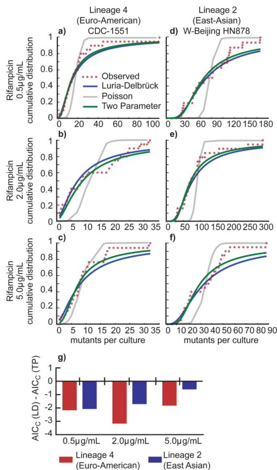
Figure 3. The cumulative distribution of drug resistant mutants from both lineages indicates that mutations do not occur after exposure to antibiotic
