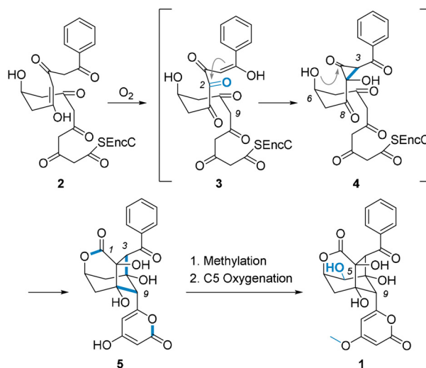
Scheme 1. Biosynthetic pathway from dihydrooctaketide 2 (EncC = enoyl-CoA carrier protein) to enterocin ( 1 ). [5–11] Oxygenation at position C2 (enterocin numbering) initiates a Favorskii-type rearrangement which proceeds via cyclopropanone 4 to precursor 5 of the natural product: Two aldol reactions establish the key bonds C3–C4 and C8–C9 of the tricyclic skeleton.
