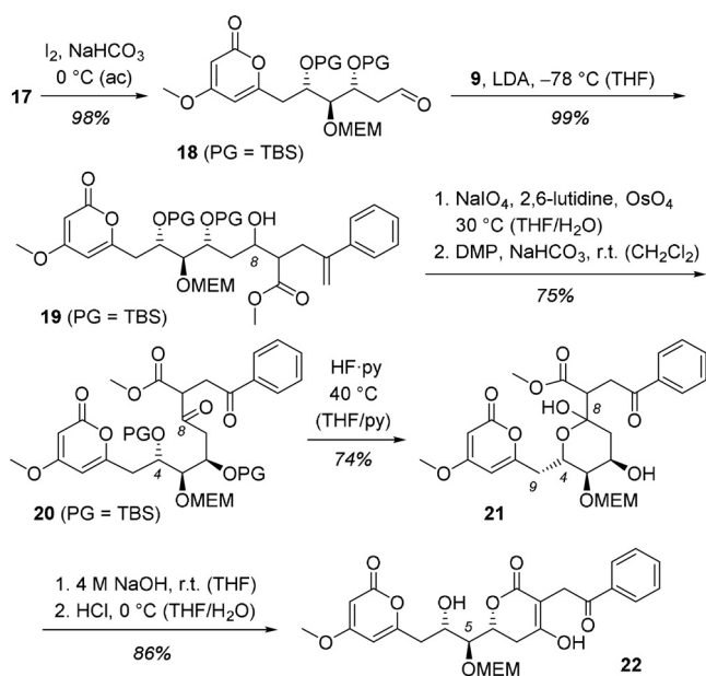
Scheme 4. Assembly of the lactone precursor 21 of enterocin by an aldol reaction of ester 9 to aldehyde 18 and subsequent functional group manipulations (DMP = Dess–Martin periodinane). Formation of hemiacetal 21 was a first indication that a substituent at carbon atom C4 can intramolecularly attack the C8 carbonyl group.
