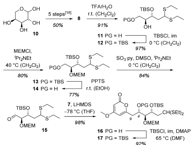
Scheme 3. Synthesis of the left-hand fragment 17 of enterocin from L-arabinose ( 10 ): An aldol addition of methoxypyronone 7 to aldehyde 15 establishes the C–C bond at positions C4 and C9 [TFA = trifluoroacetic acid, PG = protecting group, im = imidazole, PPTS = pyridinium para -toluenesulfonate, py = pyridine, LHMDS = lithium hexamethyldisilazide, DMAP = 4-( N,N -dimethylamino)pyridine].
