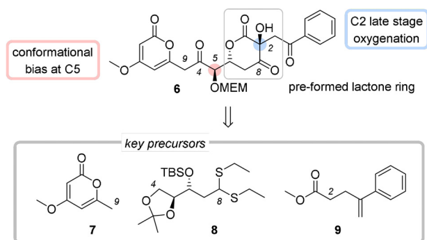
Scheme 2. Retrosynthetic disconnection and key features of the pivotal intermediate 6 (numbering as for enterocin) for a two-fold biomimetic aldol reaction (MEM = 2-methoxyethoxymethyl, TBS = tert -butyldimethylsilyl). Top: The pre-formed lactone ring and the conformational bias invoked by the stereogenic center at C5 should favor the cyclization (C8-C9 bond formation). The correct oxidation states at carbon atoms C2 and C4 were envisaged to be generated in the final steps in the synthesis of compound 6 . Bottom: Three components 7–9 comprise all carbon atoms required for the assembly of enterocin.
