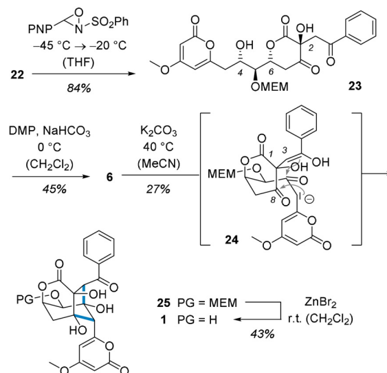
Scheme 5. Conclusion of the total synthesis of enterocin ( 1 ). Hydroxylation at C2 occurs presumably via the enol of \delta -lactone 22 . After oxidation of alcohol 23 , the formation of product 25 was observed when storing a solution of ketone 6 at room temperature. The reaction was accelerated by treatment of ketone 6 with a mild base. For further details, see the narrative.
