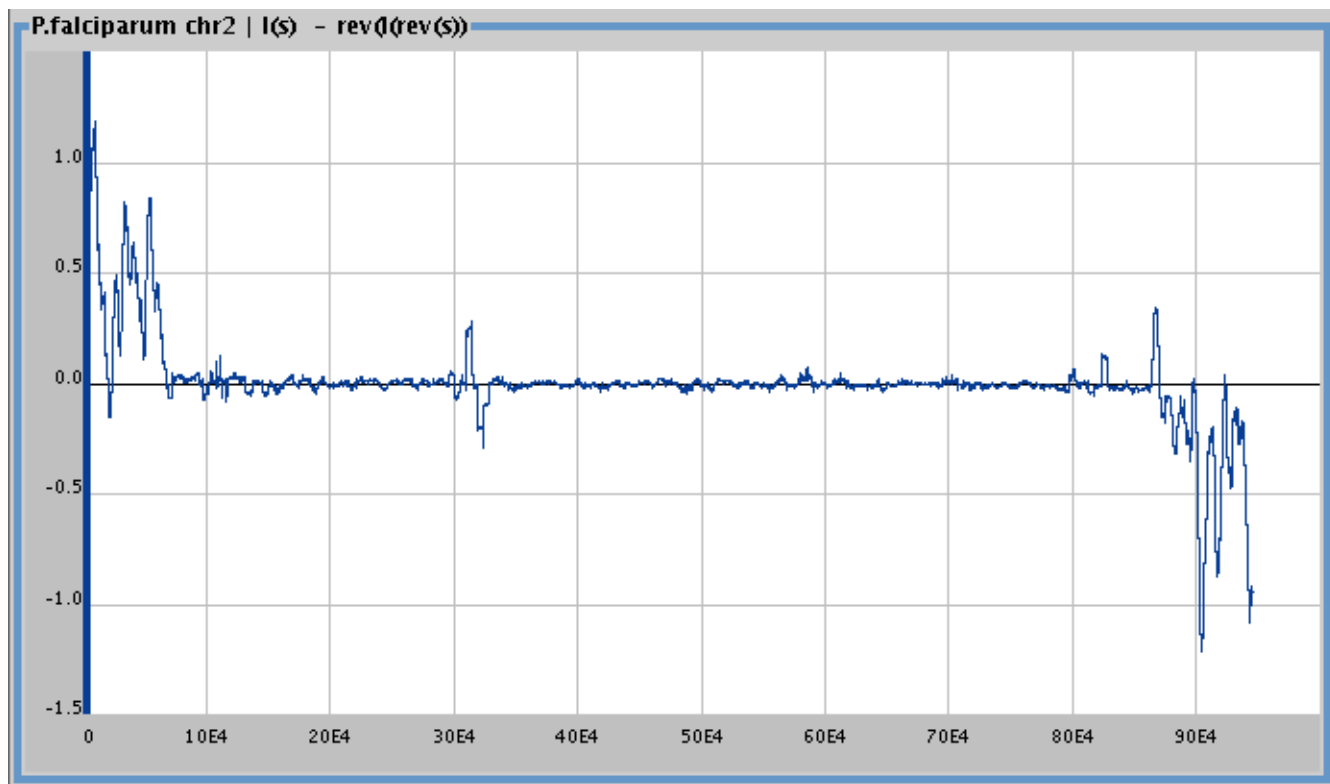
Figure 4 Plot of I(c2) - rev(I(revcomp(c2))) for chromosome 2 of P. falciparum , smoothing window 5000. Sequence highlighting the first and last reasonably long repeats within P. falciparum chromosome 2. The right to left information sequence is found for the reverse complement and is then reversed to be left to right. The resulting sequence is subtracted from left to right information sequence.
