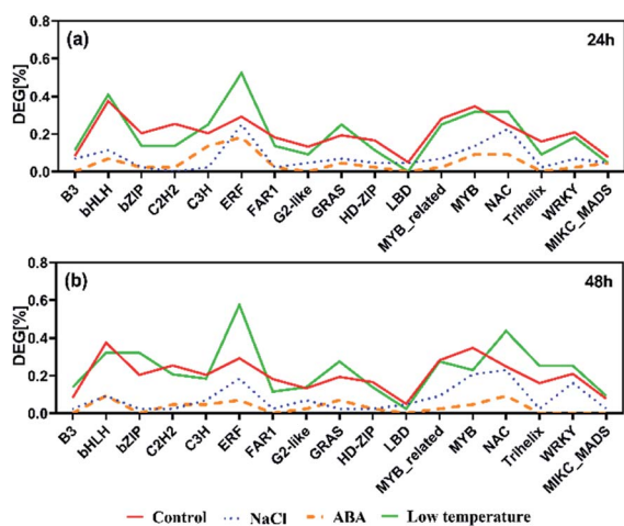
Fig. 5 The prevalence of transcription factor (TF) families after salt, ABA and low temperature stress for 24 h (a) and 48 h (b). Families with \geq 30 expressed members are shown.
