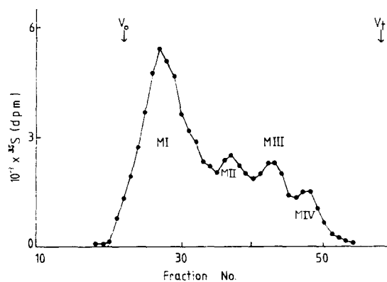
FIGURE 6 Gel filtration chromatography of sulphated macromolecules precipitated from the culture medium by (\text{NH}_4)_2\text{SO}_4 at 30% saturation. Lens cell cultures were incubated with \text{Na}_2^{35}\text{SO}_4 (500 \mu\text{Ci/ml} ) for 24 h at 37°C. The medium was removed, cooled to 4°C, and spun to remove cellular debris. Benzamidine hydrochloride (5 mM), 6-aminohexanoic acid (0.1 M), and EDTA (10 mM) were added to the concentrations indicated and (\text{NH}_4)_2\text{SO}_4 (176 mg/ml) was added slowly, with stirring. The resulting precipitate was collected by centrifugation at 80,000 g for 1 h at 4°C, resuspended in 4 M guanidine hydrochloride/50 mM sodium acetate, pH 5.8 containing the above inhibitors and dialyzed exhaustively against the same buffer at 4°C. The suspension was clarified by filtration and an aliquot chromatographed on a column of Sepharose CL-4B (1.5 × 90 cm) in 4 M guanidine hydrochloride buffer at 4°C. The void volume ( V_0 ) was 57 ml and the total volume ( V_t ) was 151 ml. For reference purposes the peaks of radioactivity have been designated MI–MIV.
