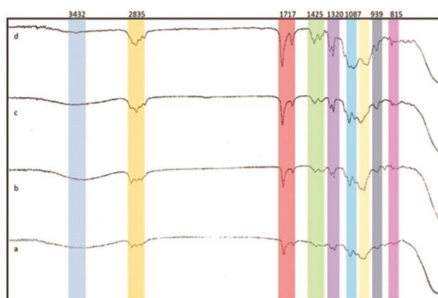
Fig. 2. FTIR spectra of the ceramic primer solution tested at different time points; a) baseline; b) one month; c) two months; d) six months.
