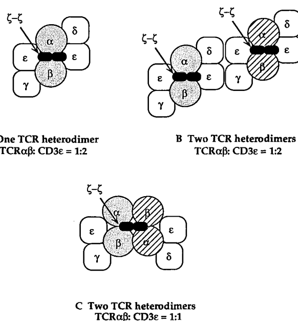
Figure 1. Three models of TCR/CD3 stoichiometry.
