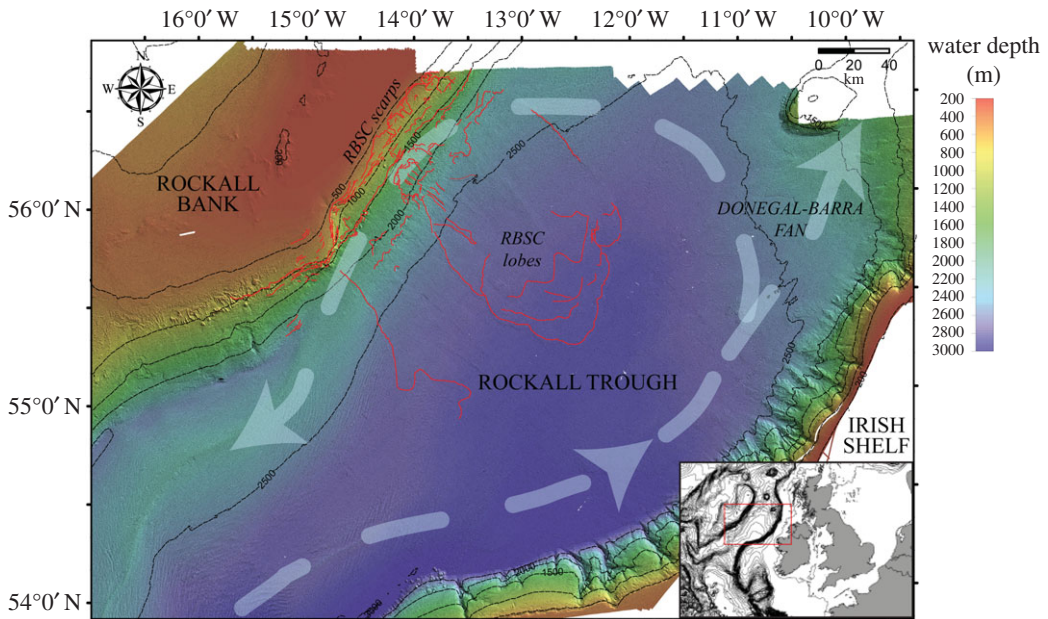
Figure 1. Multibeam bathymetry map of the Rockall Trough based on the Irish National Seabed Survey (INSS) dataset. The RBSC scarps and lobe limits are indicated with red lines. Arrows show the general oceanographic circulation. Bathymetric contours are shown with thin black lines. The map on the right-bottom corner shows the position of the RBSC with respect to Ireland and the UK. Adapted from Georgiopolou et al. [35]. (Online version in colour.)
