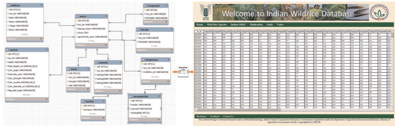
Figure 1. Schematic representation of the flow of data from the backend (MySQL) database to the frontend (JSP page) using middleware (Glassfish server) program.
