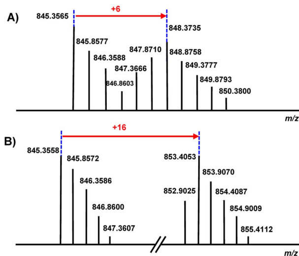
Fig. 3 (A) The MS profile of nocapeptin A (1), [M + 2\text{H}]^{2+} upon culture supplementation with [^2\text{H}_7] L-Tyr. (B) The MS profile of nocapeptin A (1), [M + 2\text{H}]^{2+} upon culture supplementation with [^2\text{H}_8] L-Trp.
