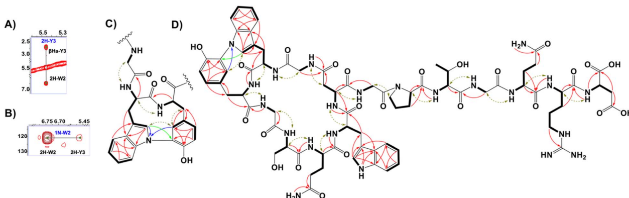
Fig. 4 (A) ^1\text{H} - ^1\text{H} NOESY spectrum highlighting the correlations between 2H-Trp2 and 2H-Tyr3 centers in nocapeptin A (1). (B) ^1\text{H} - ^{15}\text{N} HMBC spectrum showing the correlations between the 1N-Trp2 and 2H-Tyr3 in nocapeptin A (1). (C) The key NMR correlations proving the elucidated biaryl fragment ( ^1\text{H} - ^1\text{H} COSY and ^1\text{H} - ^1\text{H} TOCSY: bold lines, ^1\text{H} - ^1\text{H} NOESY: brown arrows, ^1\text{H} - ^{13}\text{C} HMBC: red arrows, ^1\text{H} - ^{15}\text{N} HMBC: blue arrows and ^1\text{H} - ^{13}\text{C} LR-HSQMBC: green arrows). (D) The complete 2D-chemical structure of nocapeptin A (1) with the key NMR correlations.
