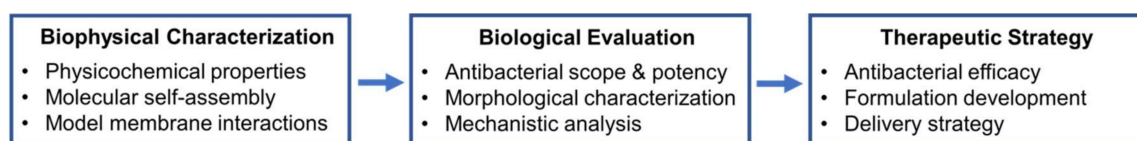
Figure 8. Overview of experimental strategy to characterize antimicrobial lipids based on integrating biophysical and biological approaches.
