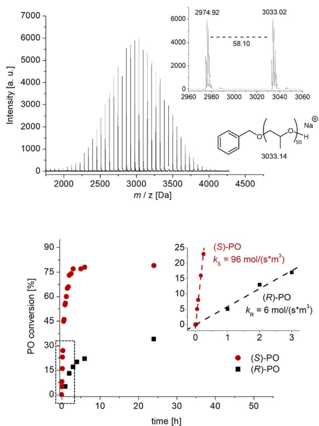
Fig. 2 Top: MALDI-ToF MS analysis of PPO prepared by the action of DBU/1 (bulk, -36 °C) with BnOH as initiator. Bottom: Polymerization kinetics using enantiopure monomer (2 M in THF, ambient, NHO/1/BnOH/PO = 1 : 2 : 5 : 2000 molar ratio).
