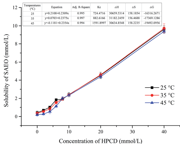
Fig. 2 Phase solubility curves and thermodynamic properties of SAEO with HPCD in water at different temperatures.
