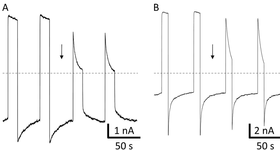
Figure 4. Records illustrating the voltage gating of (PA_{63})_7 channels and its effect on the LF_N unblocking kinetics. Before (His)_6 - LF_N addition to the cis solution, there is some gating of the channels at positive voltage pulses and very significant gating at negative voltage pulses; the latter is more marked in B than in A. The gating kinetics are such that channels that have closed at negative voltages rapidly reopen at positive voltages. After LF_N addition (arrow), blocking occurs at positive voltage pulses, but the unblocking kinetics at negative voltage pulses are convoluted with the intrinsic gating kinetics of the channels. In A, actual un-
