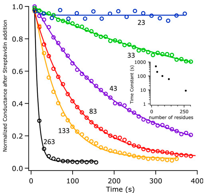
Figure 7. The rate of capture by trans streptavidin of the biotin at residue 1 of (His)_6 - LF_N constructs of various lengths, with YFP attached to the C terminus. These data come from experiments such as that depicted in Fig. 6 and are fit by single exponentials with the time constants indicated in the inset. The conductances are normalized to the value before the addition of LF_N -YFP. The voltage protocol for all of these records was +50 mV for 5 s and -40 mV for 15 s. Note that, as expected (see Results and Discussion), the shorter the length of the construct, the longer the time constant. Most significantly, the biotin at residue 1 of LF_N 1-23 is not captured by trans streptavidin, whereas that for LF_N 1-33 is slowly captured. (The LF_N 1-263 experiment was done on channels formed by the PA_{63} double mutant R178A/K214E.) The time on the abscissa is the cumulative time spent at positive and negative voltages.
