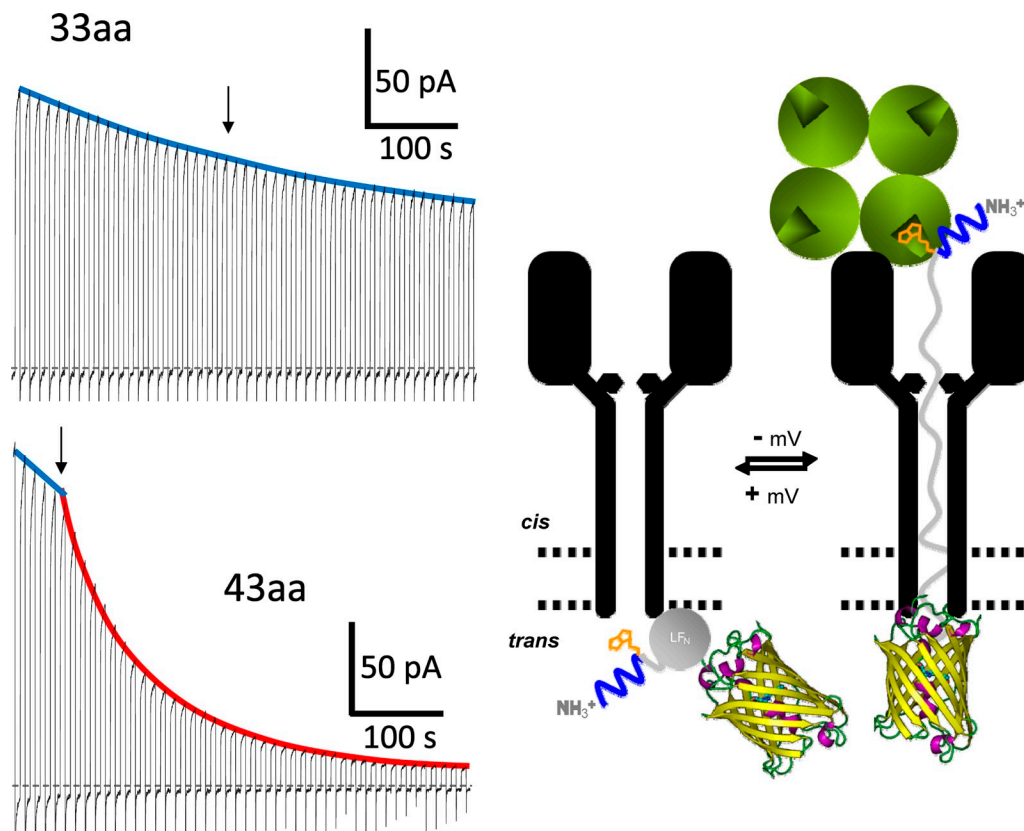
Figure 12. Example of backward translocation of a (His)_6 - LF_N construct ( LF_N 1–43 YFP with 1C biotinylated) whose N terminus reached the cis solution, and a (His)_6 - LF_N construct ( LF_N 1–33 YFP with 1C biotinylated) whose N terminus did not reach the cis solution. This is essentially the same type of experiment as the one depicted in Fig. 6, except in this case, the relevant LF_N -YFP mutant was added to the trans side and streptavidin was added to the cis side. After the (PA_{63})_7 -induced conductance had leveled off, the LF_N -YFP mutant was added to the trans side to a concentration of 240 nM, and the voltage protocol of -80 mV for 6 s and +30 mV for 5.5 s was begun. At the arrow, streptavidin was added to the cis compartment to a concentration of 1 \mu M. We see that before the addition of streptavidin, the level of unblocking was declining, having not yet reached a steady state. Most significantly, however, is that in the case of LF_N 1–43 YFP, this rate of decline increased dramatically upon the addition of the cis streptavidin, indicating that the biotin at residue 1 had reached the cis solution and could be grabbed by streptavidin, whereas in the case of LF_N 1–33 YFP, the rate of decline remained unchanged, indicating that the biotin at residue 1 could not reach the cis solution. The dashed line is the zero current level. The cartoon is virtually identical to that in Fig. 11, except that here YFP, instead of biotins, is the stopper.
