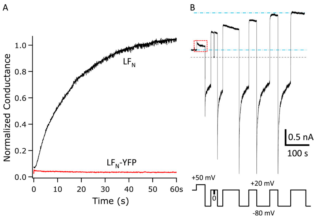
Figure 5. Demonstration that YFP attached to the C terminus of LF N prevents its translocation. (A) Before the start of the records, the (PA 63 ) 7 -induced conductance had leveled off, (His) 6 -LF N or (His) 6 -LF N -YFP had been added to the cis compartment to a concentration of 120 nM, the conductance had fallen to a fraction of the value before LF N addition, and LF N had been perfused out of the cis compartment. At t = 0 , the voltage was stepped from +20 to +50 mV. We see that LF N was readily translocated, with a half-time of \sim 10 s, whereas no translocation at all of LF N -YFP had occurred after more than 60 s. The conductance is normalized to the value before the addition of LF N or LF N -YFP. (B) The LF N -YFP record in A is a blow-up of the boxed segment of this record. The point of the rest of the record is to show that the (PA 63 ) 7 channels are still present and have not simply disappeared. The -80-mV pulses drive LF N out of the channel back to the cis side. The initial conductance when the voltage is stepped back to +20 mV is a result of the channels that were unblocked at -80 mV; the subsequent slow fall in conductance is caused by LF N still attached to those channels. The dashed blue lines mark the conductance before and after LF N -YFP block. We see that after five -80-mV pulses, the conductance has reached the value before LF N -YFP addition, thus confirming that (PA 63 ) 7 channels have not disappeared. The black dashed line is the zero current level.
