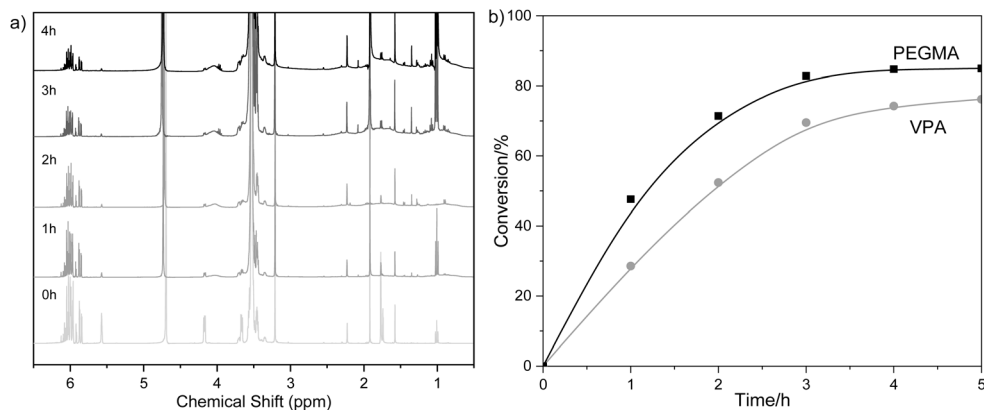
Fig. 5 (a) ^1\text{H} NMR spectra of the PV4A copolymerization in \text{D}_2\text{O} at different polymerization times, and (b) kinetic curves of the copolymerization of VPA and the PEGMA monomer.
