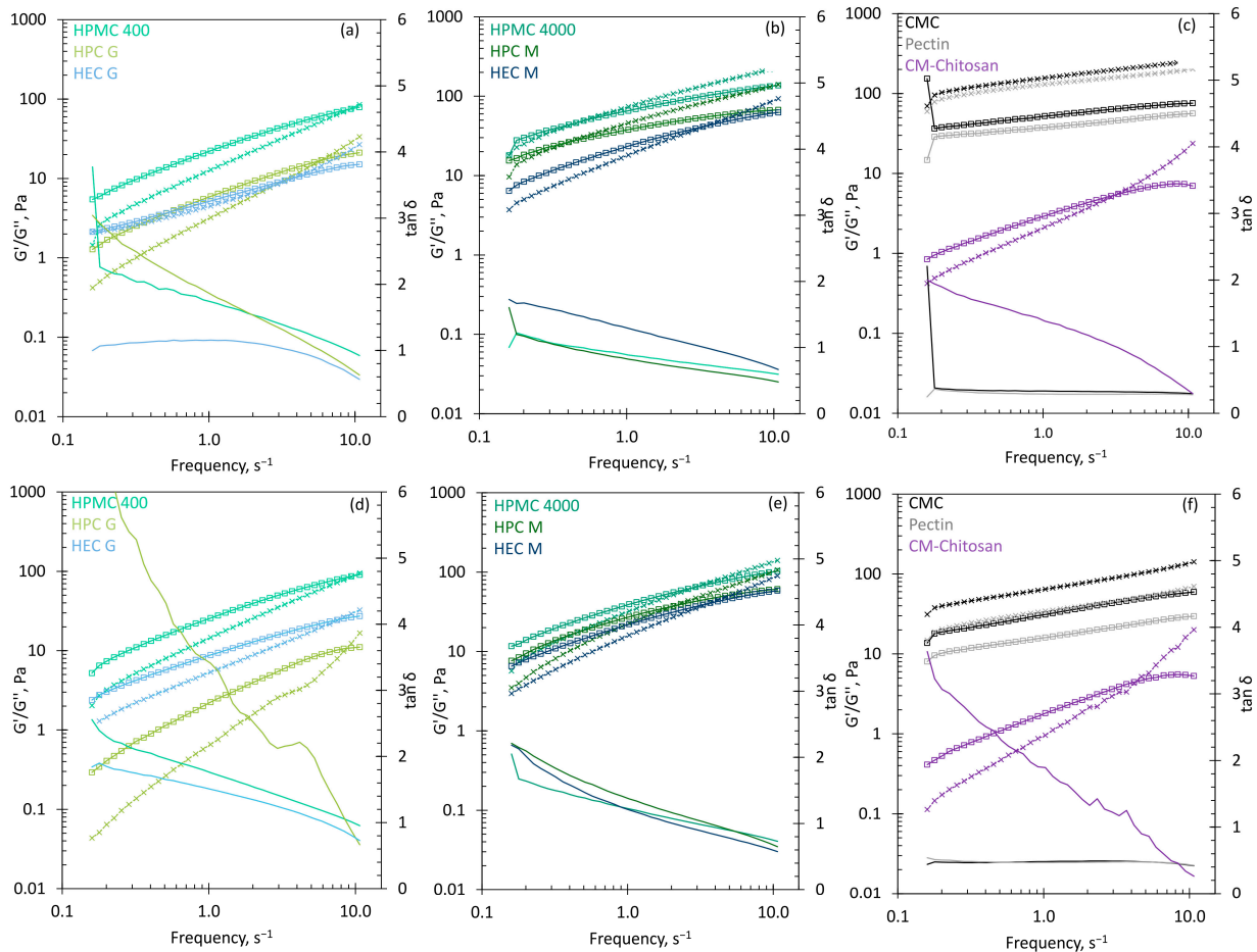
Figure 3. Frequency-dependent viscosity measurements of the mucoadhesive excipients: dotted lines with cross, elastic modulus ( G' ); solid lines with squares, viscous modulus ( G'' ); solid lines, dissipation factor ( \tan \delta ). (a) HPMC 400, HPC G, HEC G after 1 min resting time; (b) HPMC 4000, HPC M, HEC M after 1 min resting time; (c) CMC, Pectin, CM-Chitosan after 1 min resting time; (d) HPMC 400, HPC G, HEC G after 15 min resting time; (e) HPMC 4000, HPC M, HEC M after 15 min resting time; (f) CMC, Pectin, CM-Chitosan after 15 min resting time. The mean of the measurement of the three gels is shown; sd is not given for the clarity of the graph.
