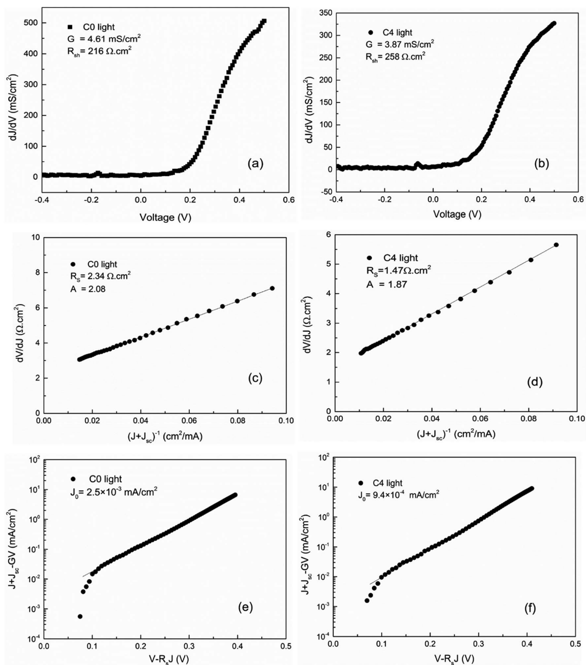
Fig. 4 Plot of dJ/dV vs. V repainted from the standard light J - V curve for CAZTSSe samples (a) C0, (b) C4, where G value was extracted from the plateau value; Plot of dV/dJ vs. (J+J_{\text{sc}})^{-1} for CAZTSSe samples (c) C0, (d) C4, where R and A value were evaluated from the intercept and slope of the linear region of the curve, respectively; semi-logarithmic plot of J+J_{\text{sc}}-GV vs. V-R_sJ for CAZTSSe samples (e) C0, (f) C4, where J_0 value was obtained from the intercept of the curve.
