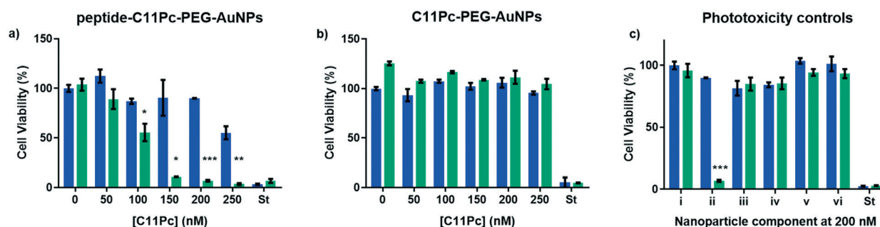
Fig. 4 Cell viability of A549 cells treated with a) peptide-C11Pc-PEG-AuNPs, b) C11Pc-PEG-AuNPs or c) i) media, ii) peptide-C11Pc-PEG-AuNPs, iii) FITC- \beta AAEYLRLK, iv) FITC-PEG-AuNPs, v) peptide-PEG-AuNPs and vi) FITC-C11Pc-PEG-AuNPs either with (green) or without (blue) irradiation. Where C11Pc was not present, cells were treated with 200 nM FITC. St = positive control of staurosporine. Error bars represent SE ( n = 3 ). Statistically significant differences are indicated by * at P \leq 0.05 , ** at P \leq 0.01 , *** at P \leq 0.001 , obtained using a two-tailed Student's t -test.
