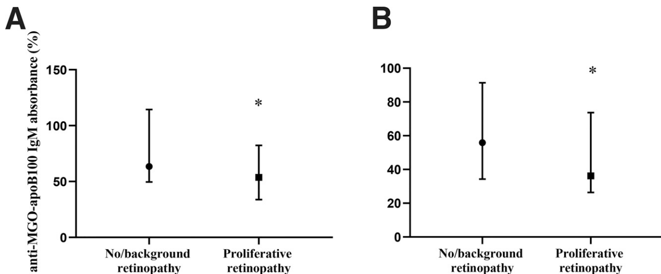
Figure 2— Levels of anti-MGO-apoB100 (A) and anti-MGO-p5 (B) in type 1 diabetes with no/background retinopathy ( n = 49) and proliferative retinopathy ( n = 34). The values are presented as median (IQR). Absorbance was measured at 405 nm and is presented as absorbance units in percentage compared to control plasma pool. * P < 0.05 (Kruskal-Wallis test).
