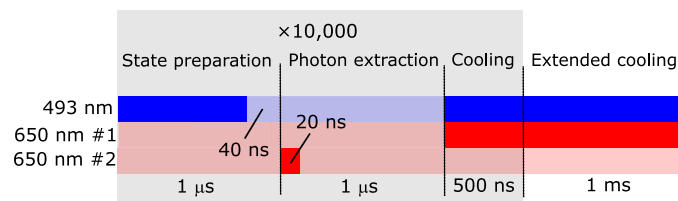
Fig. 6. Experimental pulse sequence. The experimental pulse sequence showing the timing of the laser beams used to state prepare, extract a single photon, and Doppler cool the ion. The parts of the sequence contained in the gray shading are repeated 10,000 times before an extended cooling cycle is performed.
