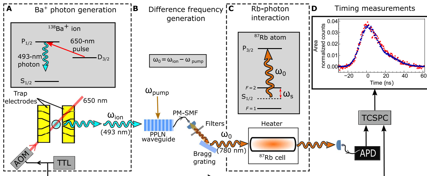
Fig. 2. Experimental schematic of photon production from a ^{138}\text{Ba}^+ ion, QFC, and photonic slowing in a warm neutral ^{87}\text{Rb} vapor. (A) The energy levels of ^{138}\text{Ba}^+ and schematic showing the ion confined in a segmented blade trap. A TTL pulse-activated AOM controls a 650-nm excitation light. (B) The QFC setup including a PPLN waveguide. Converted light, \omega_0 , is at the difference frequency between photons emitted from the ion at \omega_{\text{ion}} and pump photons at \omega_{\text{pump}} . The output of the PPLN is fiber coupled to a polarization maintaining single-mode fiber (PM-SMF). A series of filters and a Bragg grating filter out pump light and unconverted 493-nm light, which reduces the amount of anti-Stokes noise. (C) A ^{87}\text{Rb} energy level diagram and a vapor cell housed inside a heater through which converted single photons pass. (D) Photons are detected on an APD, and a TCSPC collects the arrival time of the photons with respect to the TTL sent to the AOM. As an example, single-photon temporal shapes at 493 nm (blue circles) and frequency-converted photons after passing through the cell at room temperature (red circles) are shown.
