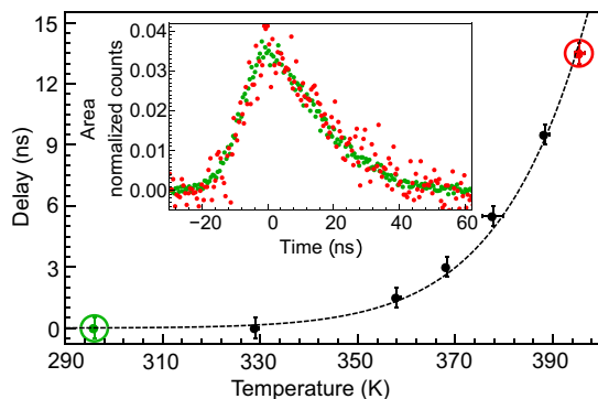
Fig. 5. Delay of the frequency-converted photons emitted from the trapped \text{Ba}^+ ion after passing through a ^{87}\text{Rb} vapor cell as a function of the cell's temperature. The dashed theory curve is a scaled version of Eq. 3 to account for N . The temperature and delay error bars are due to temperature fluctuations over the course of the experiment and the bin width of the histogram photon arrival time data, respectively. Inset: Overlap of temporal shapes of photons transmitted through a 296-K room temperature cell (green circles) and a 395-K cell (red circles). The relative delay between the two traces has been removed to allow for comparison.
