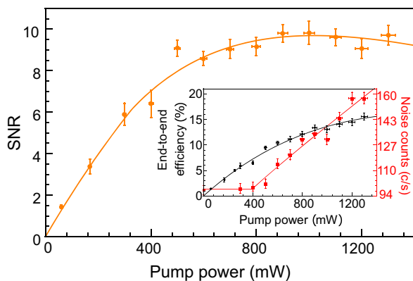
Fig. 3. SNR measured after filtering of the frequency-converted ion signal. The orange curve is the SNR given the measured conversion efficiencies and noise at each pump power. Inset: Measured conversion efficiency (black) and measured noise counts (red) on the APD as a function of pump power. The black curve is a theoretical fit to the efficiency data, and the red curve is an empirical fit to the noise.
