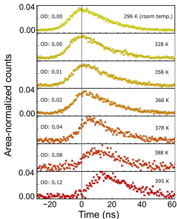
Fig. 4. Area-normalized temporal photon shapes. Area-normalized temporal shapes of frequency-converted photons that have passed through a warm ^{87}\text{Rb} vapor cell. The ^{87}\text{Rb} vapor cell temperature is set to the values indicated. The optical density (OD) of the warm vapor is stated for each temperature, at a frequency \omega_0 , and using the same atomic density, N , used to fit the delay curve in Fig. 5.
