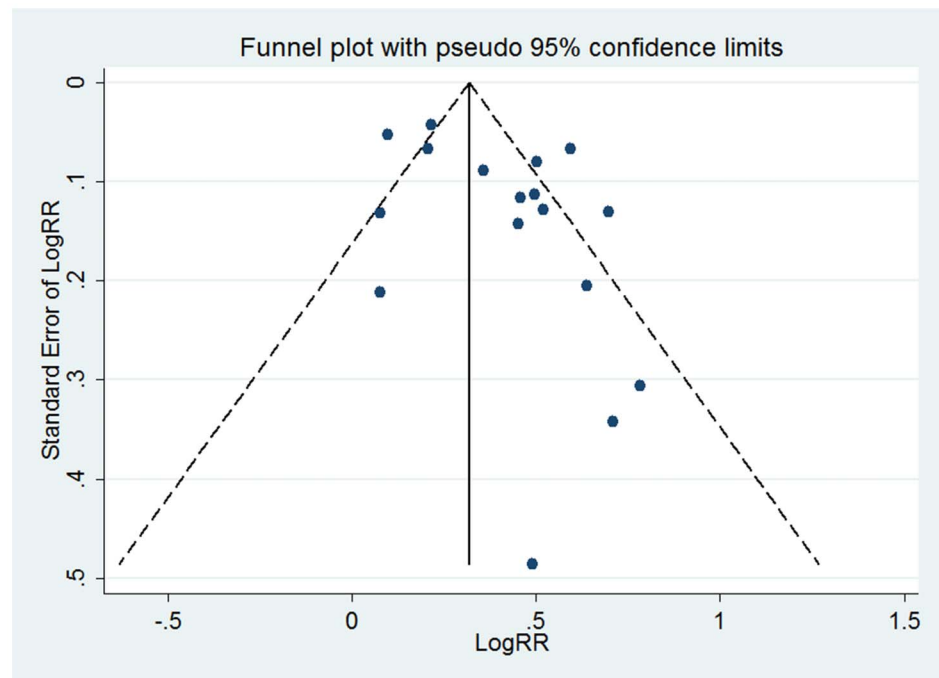
Figure 5. Funnel plot of studies reporting categorical data of hyperuricemia and risk of incident hypertension.
