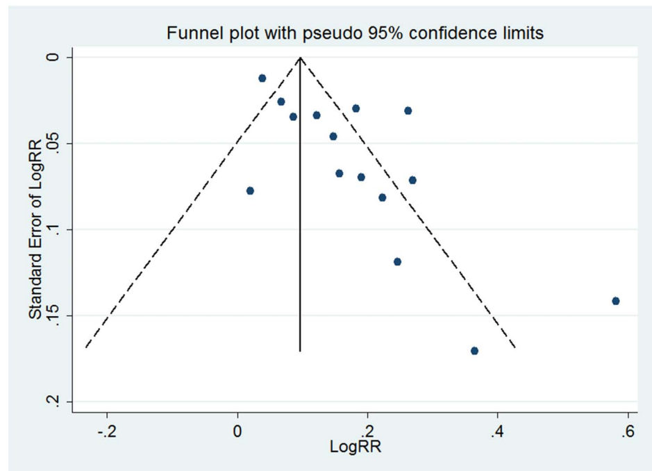
Figure 6. Funnel plot of studies reporting continuous data of hyperuricemia and risk of incident hypertension.
