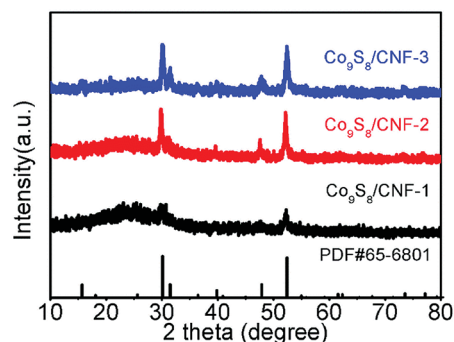
Fig. 1 XRD pattern of the \text{Co}_9\text{S}_8/\text{CNF} samples.
