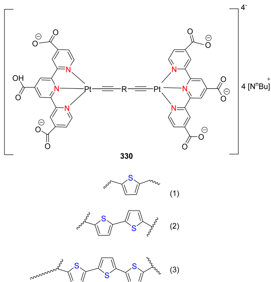
Fig. 32 Platinum complexes used in dye sensitizer solar cells (DSSCs).
