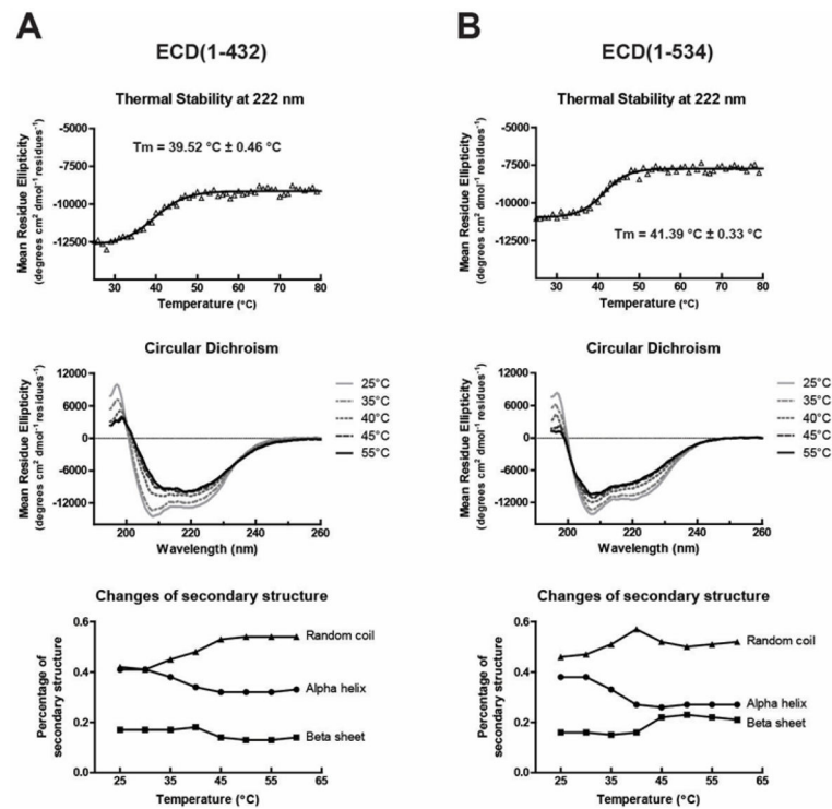
Figure 2. Thermal stability study of ECD fragments by CD. T m of (A) ECD(1–432) and (B) ECD(1–534) were measured by the change of CD signal at 222 nm from 25 to 80 °C (upper panel). The T m was determined by nonlinear least squares fitting. In the middle panel, only spectra obtained at 25 (pale grey solid line), 35 (grey dot-dashed line), 40 (grey dotted line), 45 (dark grey dashed line), and 55 °C (black solid line) are displayed for clarity. In the bottom panel, the percentage changes of the random coiled (triangle), \alpha -helix (dot), and \beta -sheet (square) composition were estimated by DichroWeb and plotted as a function of temperature.
