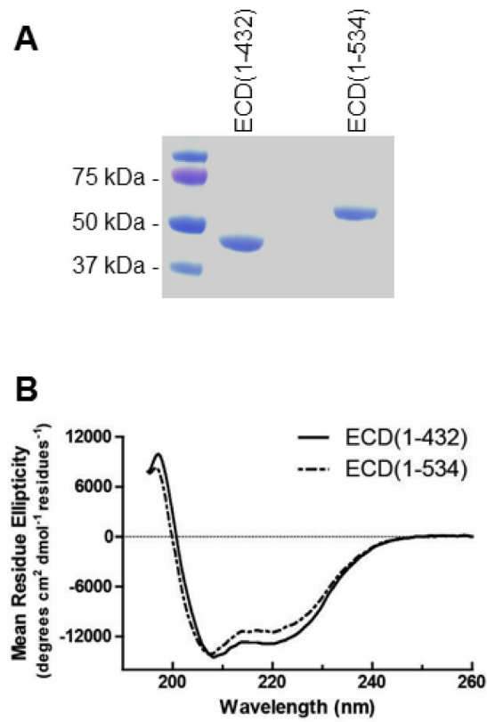
Figure 1. Characterization of ECD(1–432) and ECD(1–534) samples. (A) Purity shown with Coomassie-stained SDS-PAGE. (B) Secondary structure measured with circular dichroism at 25 °C(B).
