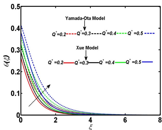
Fig. 6 Curve of \theta(\xi) in relation to Q^* .
