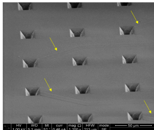
Figure 4. Fabricated NOA81 microsieve using spin-coating shows a successful replica with the nanometer high features of the original \mu\text{SEA} (yellow arrows).
