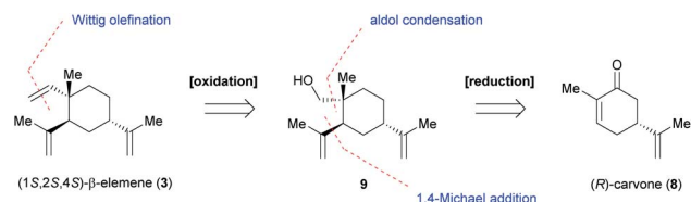
Scheme 2 Retrosynthetic analysis of (1 S ,2 S ,4 S )- \beta -elemene.
