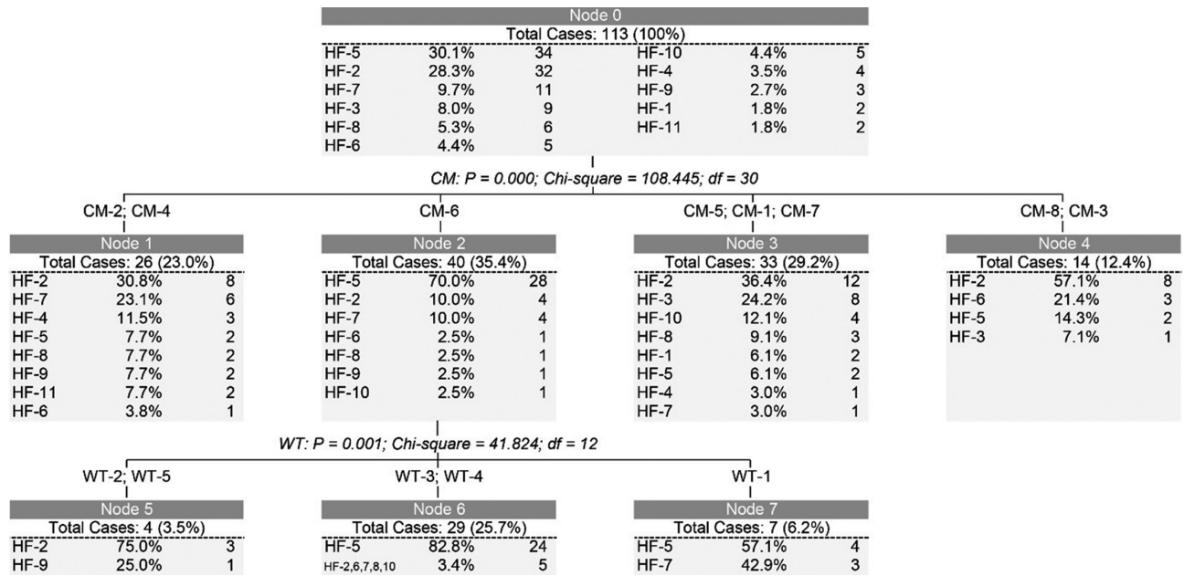
Fig. 2. Classification tree.
