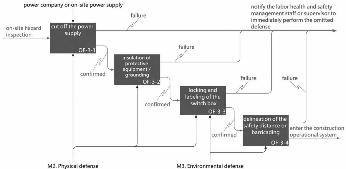
Fig. 6. Flowchart of on-site hazard inspection.
