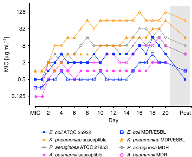
Fig. 3 Serial passage resistance induction of AA139 against susceptible and MDR Gram-negative bacteria. MIC values for AA139 before and after each of 20 passages (1 passage per 24 h, n = 1 ) treated with 0.5 \times \text{MIC } \mu\text{g mL}^{-1} (of previous passage). Bacteria that grew at the highest concentration of AA139 on the final passage were passaged a further 3 times on drug-free agar plates before determining the final MIC by BMD (“Post”, gray shading). Tabulated MIC values for AA139 and arenicin-3 are presented in Supplementary Table 7. Strains used in this study are detailed by (#) in Supplementary Data 3.
