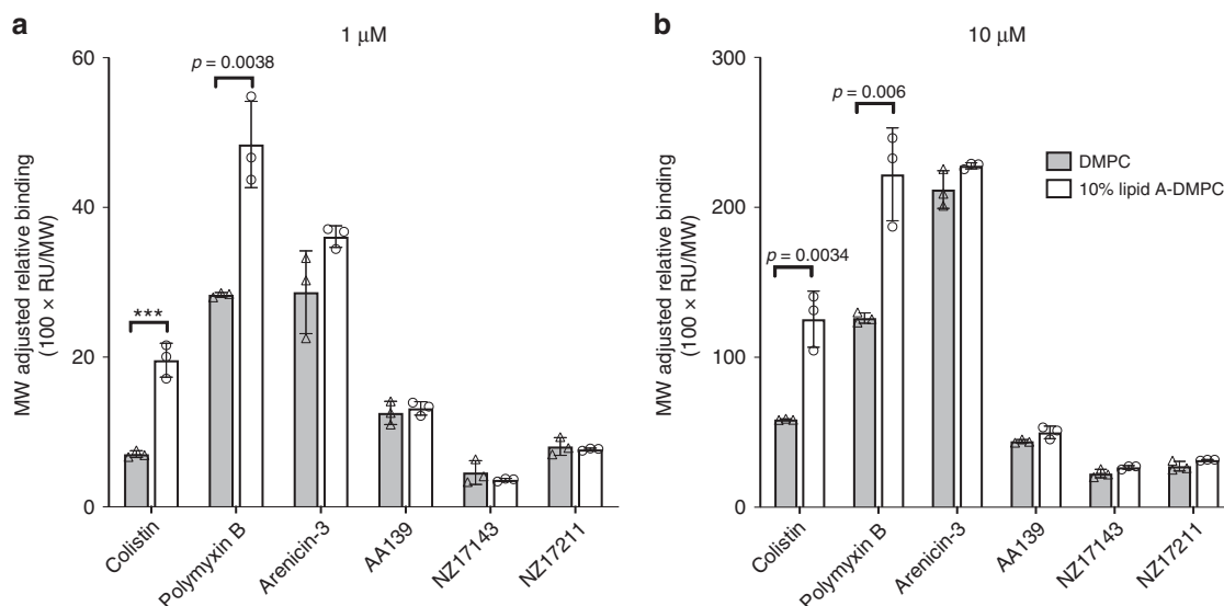
Fig. 2 Binding of arenicin-3 variants to lipids as monitored by SPR. Comparison of the propensity of arenicin-3, AA139, NZ17143, NZ17211, and other membrane binding antimicrobials, colistin and polymyxin B, to bind to various model membrane lipid systems. DMPC (gray) is compared to DMPC with 10% E. coli lipid A (white) at 1 \mu\text{M} a and 10 \mu\text{M} b . Mean data of n = 3 per test group is plotted with error bars shown as SEM. Significant difference in binding affinities can be seen for colistin and polymyxin B between the two lipid systems; however, not for arenicin-3 variants. Statistical comparison performed with Prism 8 using Student's t -test, all differences between means with p < 0.01 are indicated; ***p \leq 0.001 . RU response unit, MW molecular weight. Source data are provided as a source data file.
