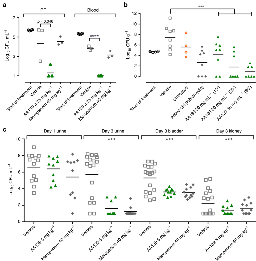
Fig. 5 In vivo peritonitis, pneumonia and UTI murine models for AA139. a Peritonitis model dosed at 3.75 mg kg -1 against MDR E. coli AID#172 (inoculated in the lateral lower quadrant of the abdomen by single i.v. dose) with CFU mL -1 measured in the peritoneal fluid (PF) and the blood after 5 h post infection ( n = 4 for start of treatment groups and n = 3 for other groups). b P. aeruginosa pneumonia model treated with aerosolized AA139 for 10, 20, or 30 min duration in an aerosol exposure chamber at 2, 12, and 24 h post infection. The bacterial load (CFU g -1 lung tissue) was measured at 34 h post infection ( n = 4 for start of treatment group, n = 7 for AA139 30 min treatment group and n = 8 for other groups). c Bacterial load (CFU mL -1 ) in the urine of UTI murine model infected with ESBL producing E. coli DSA 443 before treatment (day 1), and bacterial load (CFU mL -1 ) in the urine, bladder, and kidney after last treatment (day 3). Animals were treated twice-daily with AA139 at 5 mg kg -1 or meropenem at 40 mg kg -1 i.v. ( n = 12 ). Horizontal bar indicates geometric mean burden of each treatment. Statistical comparison performed with Prism 8 using one-way ANOVA, Dunnett's multiple comparisons test, and all differences between means with p \leq 0.05 are indicated: *** p \leq 0.001 ; **** p \leq 0.0001 . Source data are provided as a source data file.
