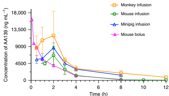
Fig. 6 The pharmacokinetic profile across species of systemically administered AA139. Plasma or serum AA139 concentration in mouse, monkey and minipig over time after the initiation of a 10 mg kg -1 dose (i.v. continuous infusion over 2 h, or i.v. single bolus injection). Mean values with error bars shown as SEM (mouse i.v. infusion n = 6 , mouse i.v. bolus n = 3 , monkey n = 2 , minipig n = 2 ; male and female combined for all species) are plotted using Prism 8. Source data are provided as a source data file.
