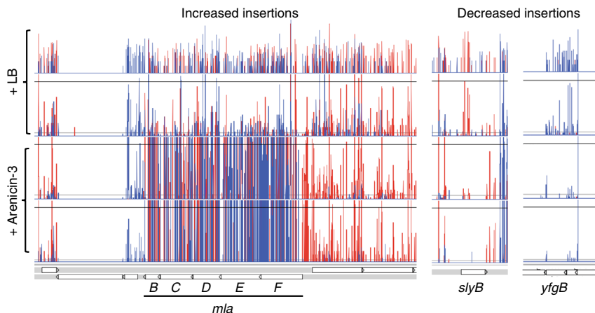
Fig. 4 TraDIS reads representing transposon insertions across the mla operon (B-F), slyB and yfgB in UPEC. The arenicin-3-treated library is represented by the bottom two rows and the controls with LB only, the top two rows. Insertion positions of Tn5 mutations at each bp are represented by vertical lines, the depth represented by the height of the line and the direction of insertion, the color (forward and reverse are red and blue, respectively) across the entire mla operon. Note, mlaA is not shown here as it is located separately but also displayed the same pattern of insertions.
