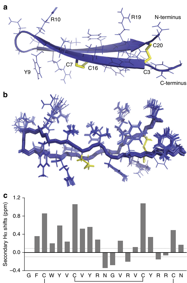
Fig. 1 3-Dimensional NMR solution structure of arenicin-3. a Structure displayed in cartoon form showing the classic \beta -hairpin assembly created by anti-parallel \beta -sheets and two stabilizing disulfide bonds (yellow) across the sheet, key residues and the N and C terminus labeled for orientation. b Overlay of 20-lowest energy structures, aligned by backbone. c Secondary H \alpha shifts (variation from random coil). Structure deposited as PDB 5V0Y and BMRB 30259 and images created using PyMol. Structural refinement statistics are displayed in Table 1.
