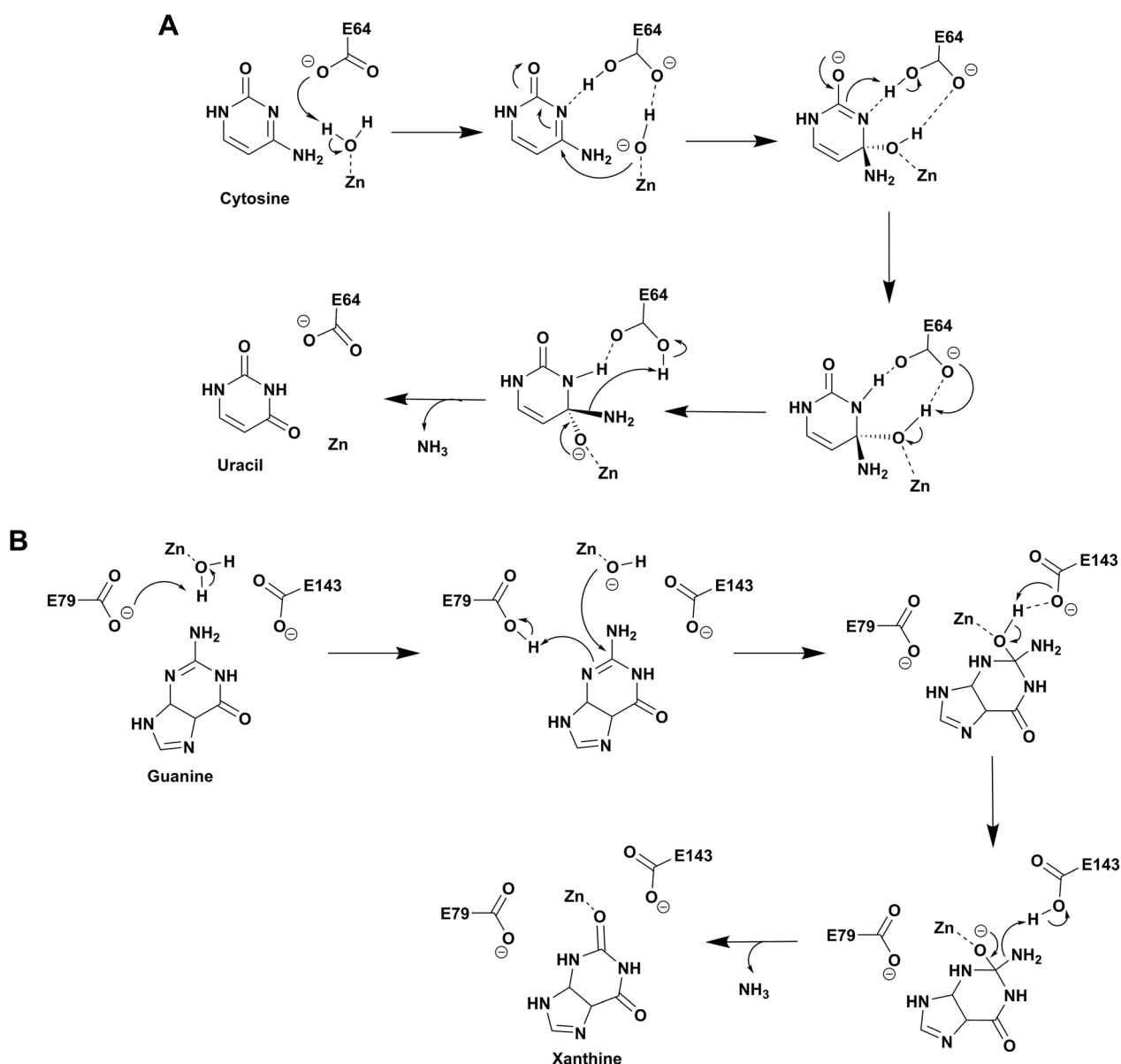
Scheme 2 Proposed catalytic mechanism involving one glutamic acid residue in \gamma CD (A) and two glutamic acid residues in NE0047 (B).
