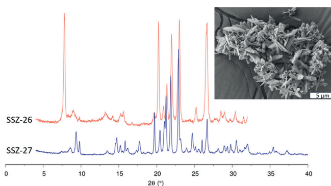
Figure 2. XRPD pattern for SSZ-26 ( CON ) and SSZ-27, both as-synthesized. The inset shows an SEM image of as-synthesized SSZ-27. Note that the SSZ-27 sample shown may contain an SSZ-26 impurity (see text).
