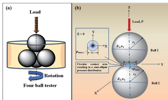
Scheme 2 (a) Representational image showing four balls placed in a sample holder. (b) Contact between two interacting balls in a four-ball tester.
