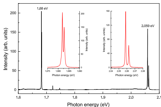
Figure 5. Typical photoluminescence spectrum of diamonds synthesized in the \text{Mg}_{0.9}\text{-Ge}_{0.1}\text{-C} system. The spectrum was recorded at 80 K with the 532-nm excitation for a diamond crystal produced in the \text{Mg}_{0.9}\text{-Ge}_{0.1}\text{-C} system at 7 GPa and 1700 °C. The insets show ZPL regions of the 2.059 and 1.68 eV centres.
