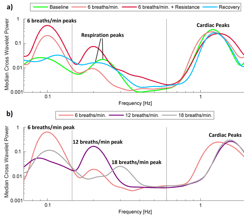
Figure 6. Median of the time-averaged CWP of BP and SAS LEFT signals recorded in all subjects for (a) procedure 1 and (b) procedure 2. Various line colours correspond to different stages of procedure.
