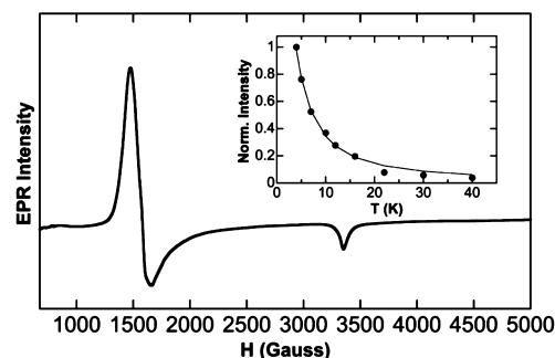
Figure 2. 10 K EPR spectrum of 1 in THF generated from reaction of FeCl 3 with MeMgBr. Inset shows the temperature-dependent EPR intensity of 1 and Boltzmann fit to the Curie law to give an axial ZFS parameter of D = 6.5 \pm 0.5 \text{ cm}^{-1} .
