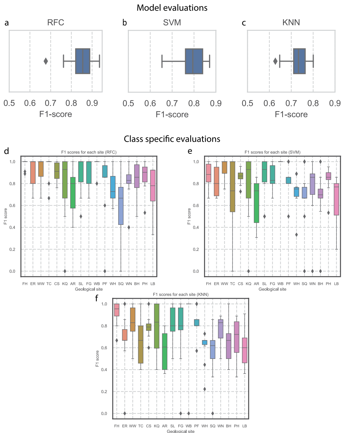
Figure 6. Evaluation of machine learning classifiers. (a–c) Distribution of F1 scores from 100-fold cross-validation for Random Forest, Support Vector Machine and K nearest neighbours, respectively. (d–f) Distribution of F1-scores for each source for Random Forest, Support Vector Machine and K nearest neighbours, respectively.
