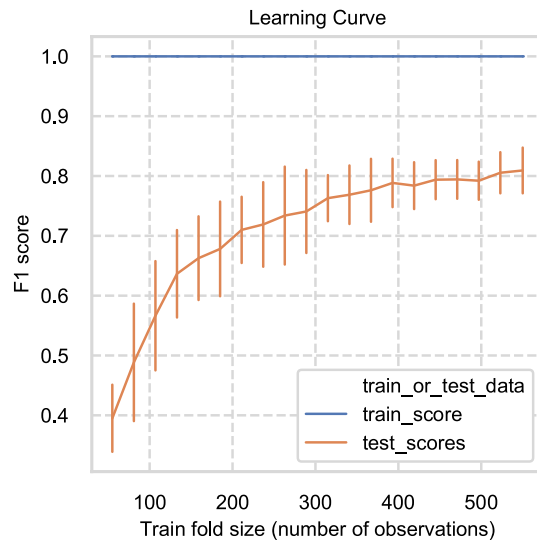
Figure 9. Learning curve shows F1 score for train and test data against number of observations in training data.
