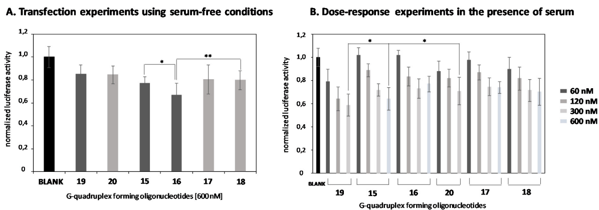
Figure 8. Gene transfection studies targeting Renilla luciferase mRNA without using lipofectamine in serum-free conditions (A). Modified and unmodified antisense conjugates (15–18) and (19, 20) were used at 600 nM. (B) Dose-response transfection experiments using several concentrations (60, 120, 300 and 600 nM) in the absence of lipofectamine. G4_(19, 20) were used as controls. Data were means \pm SD of three to six independent experiments. A regular two-way ANOVA variance analysis, combined with Bonferroni post-test for multiple comparisons, was evaluated (* p < 0.05 and ** p < 0.01 ).
