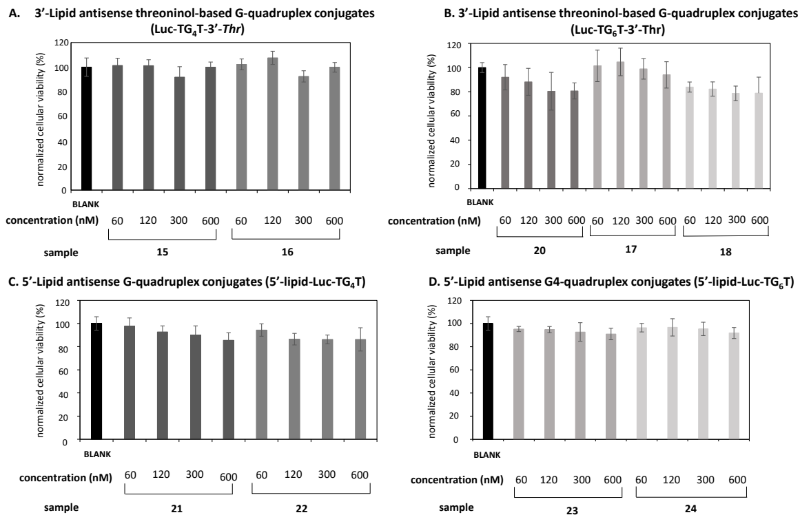
Figure 6. Cytotoxicity analysis of antisense conjugates containing four Gs (A,C) and six Gs (B,D). A lipid threoninol-based modification at the 3'-termini were introduced (A,B); a lipid modification (C8, C14) was introduced at the 5'-termini (C,D). Four concentrations of antisense conjugates, ranging from 60 nM to 600 nM, were used. All antisense conjugates were incubated up to 24 h at 37 °C. Data were means \pm SD of three independent experiments.
