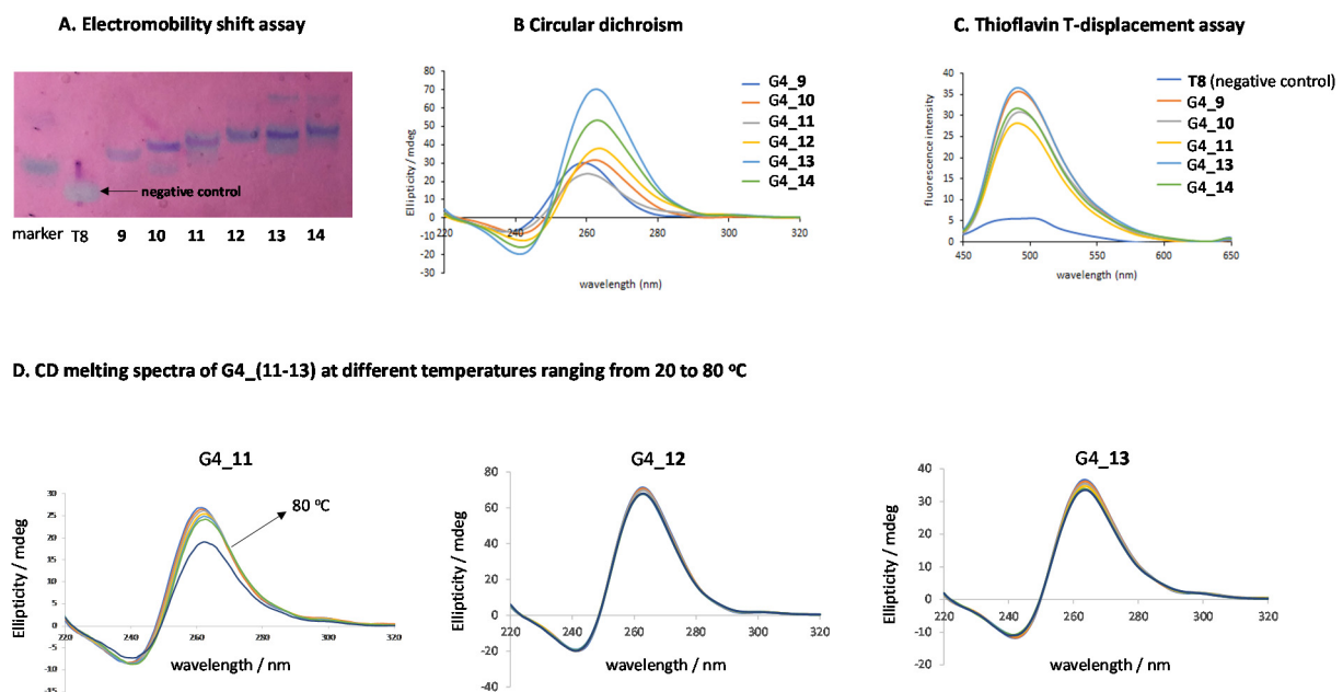
Figure 5. Native PAGE analysis, circular dichroism (CD), CD melting spectra, and Thioflavin T (ThT)-displacement assay of G-quadruplex forming oligonucleotides G4_9-14. (A) Native 20% polyacrylamide gel electrophoresis analysis of G-forming oligonucleotide conjugates (9-14) in 1X PBS supplemented with 100 mM KCl. A mixture of bromophenol blue and xylene cyanol was used as a marker. T8 is an oligonucleotide containing 8 thymidines that was used as a negative control as it is unable to form a quadruplex and indicate the position of a single-stranded 8-mer. (B) CD spectra measured at 20 °C showing positive and negative bands at 264 and 240 nm, respectively. This confirms the presence of a parallel G-quadruplex construct. G-constructs were obtained in 10 mM sodium cacodylate, 110 mM NaCl buffer; (C) ThT displacement assay shows the emitted fluorescence of ThT probe when bounded to G-quadruplex structures. A T-rich oligonucleotide (T8) was used as a negative control; (D) CD melting spectra at several temperatures ranging from 20 to 80 °C with a heating rate of 1.0 °C min -1 . All conjugates showed remarkable stabilities except, for G4_11, which had a band intensity that was slightly reduced.
