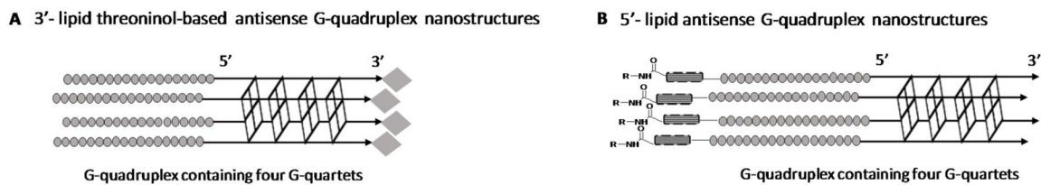
Figure 4. G-quadruplex forming oligonucleotide conjugates prepared in this study. (A). Lipid threoninol-based modifications were introduced at the 3'-termini of the G-rich sequence and (B). Lipid amino lipids were introduced, modifying the 5'-termini of the G-rich sequence.
