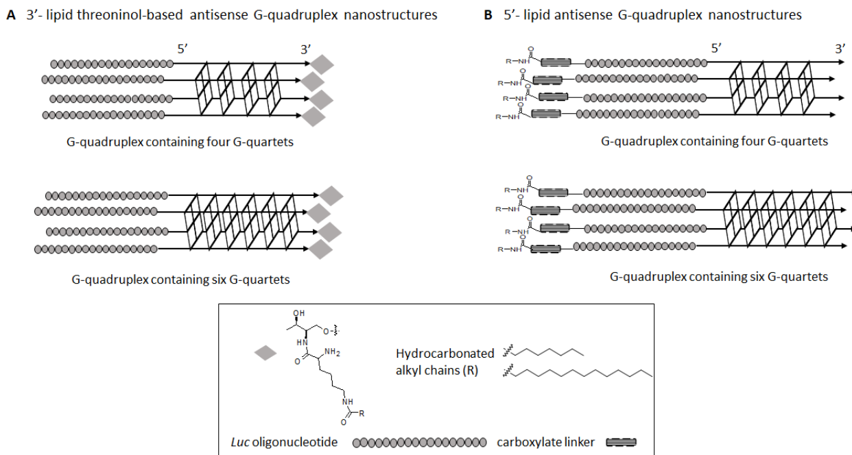
Figure 1. Two series of G-quadruplex forming oligonucleotide conjugates containing four and six G-quartets were engineered: (A) a threoninol-based building block modified with two lipids of different length (C8 and C14) was introduced covalently at the 3'-termini of a G-rich oligonucleotide sequence and (B) two hydrocarbon lipids of different length (C8 and C14) were introduced at the 5'-termini of a G-rich oligonucleotide sequence using a carboxylate linker. An 18-mer phosphorothioate ( Luc ) oligonucleotide was also attached at the 5'-termini of the G-rich sequence oligonucleotide.
