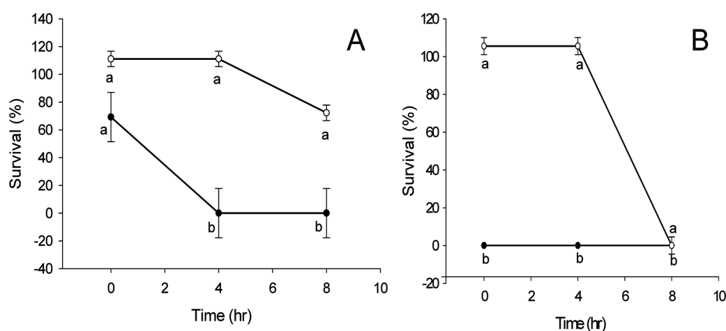
Fig. 4. Time course of the survival of Acremonium charticola (—●—) and Rhizopus oryzae (—○—). A, Viability of fungi after exposure to simulated gastric juice at pH 2; B, Viability of fungi after exposure to bile solutions 2%. Survival is presented as percentage of surviving population (cfu/mL) at different sampling times relative to initial population (cfu/mL). a,b Values with different letters within the same hour were significantly different ( p < 0.05 ).
