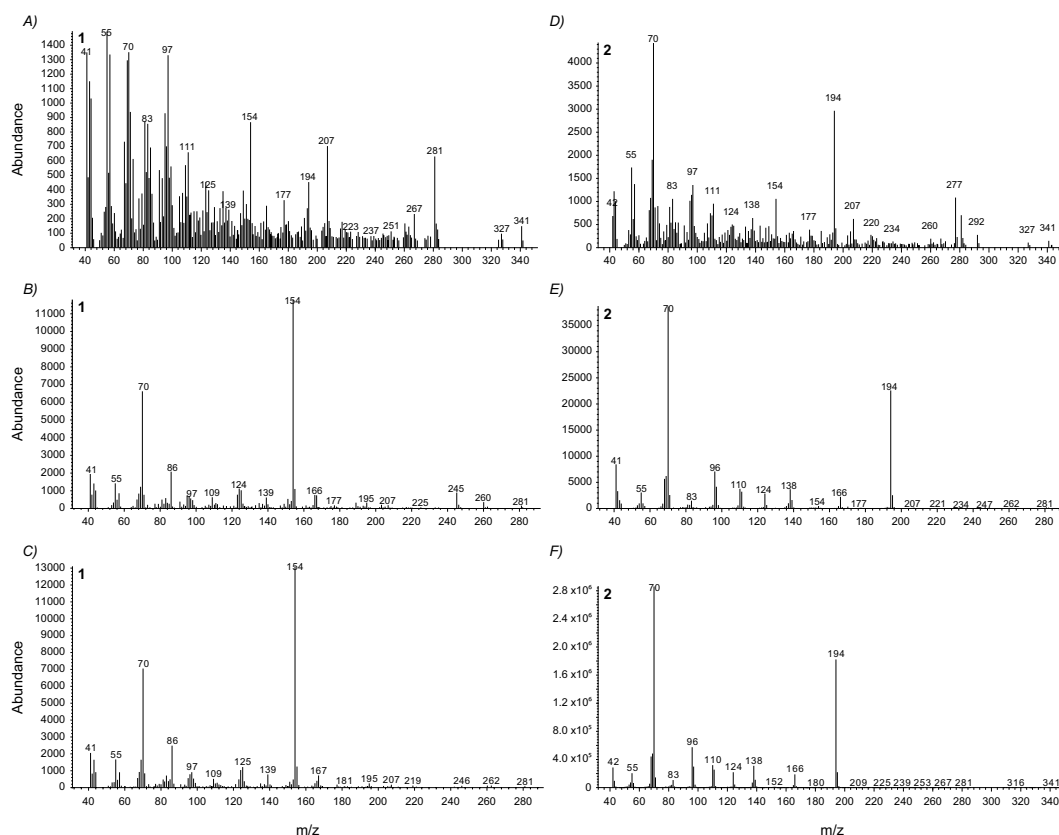
Figure 3. Mass spectra (electron impact, EI) for cyclic dipeptide 1 (1) for: S. virgatus (A), S. merriami (B), and the reference standard compound cyclo(L-Leu-L-Pro) (C). Mass spectra for cyclic dipeptide 2 (2) for: S. virgatus (D), S. merriami (E), and the reference standard compound cyclo(L-Pro-L-Pro) (F).
