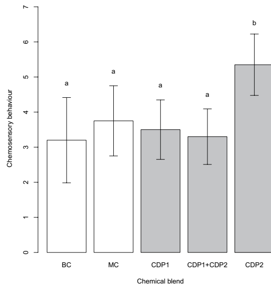
Figure 4. Chemosensory behaviour (number of tongue flicks, lip smacks, and substrate lickings of the pebble) of 20 male S. virgatus in response to a blank control (BC; an unscented pebble) and each of four different chemical blends: MC: matrix control; CDP 1: cyclic dipeptide 1, cyclo(L-Leu-L-Pro); CDP 2: synthesised cyclic dipeptide 2, cyclo(L-Pro-L-Pro); CDP1 + CDP2: a blend of CDP1 and CDP2 in equal amount. All blends included a matrix of the three most common saturated fatty acids in Sceloporus , in representative proportions, an acetone carrier and a non-volatile binding agent (PEG; see Methods). Shown are means \pm 1 S.E. Different letters denote significantly different groups.
