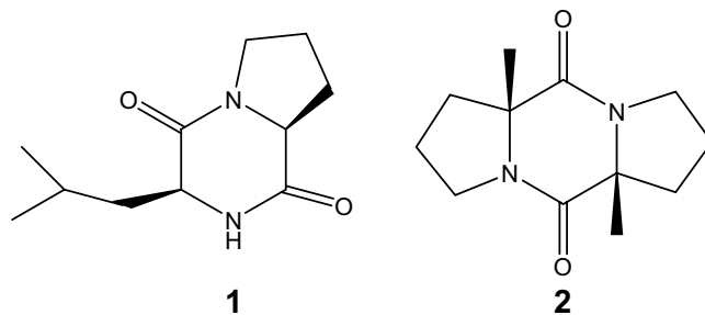
Figure 1. Chemical structures of commercially available cyclic dipeptide 1, cyclo(L-Leu-L-Pro) (1), and synthesised cyclic dipeptide 2, cyclo(L-Pro-L-Pro) (2).
