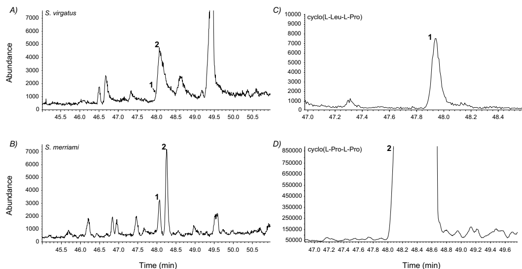
Figure 2. Post-run selected ion chromatogram (SIC), with m/z 70, from the lizard femoral gland extract of S. virgatus (A), S. merriami (B) and the reference standard compounds cyclic dipeptide 1 (C), and cyclic dipeptide 2 (D). Cyclic dipeptide 1, identified as cyclo(L-Leu-L-Pro), with retention time (Rt) 47.99 min and cyclic dipeptide 2, identified as cyclo(L-Pro-L-Pro), with Rt 48.12 min, are not fully resolved in S. virgatus but exhibit characteristic mass spectra as seen in other congeners, e.g. S. merriami 22 (B)—shown here for comparison purposes—where they occur at higher concentrations. Peak areas for cyclic dipeptide 1 were 0.09 \times 10^6 and 0.26 \times 10^6 for S. virgatus and S. merriami , respectively. Peak areas for cyclic dipeptide 2 were 0.27 \times 10^6 and 1.1 \times 10^6 for S. virgatus and S. merriami , respectively.
