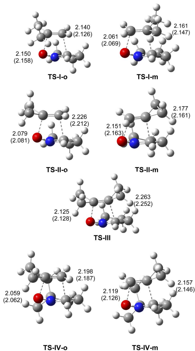
Fig. 3 \omega B97X-D/6-311G(d,p) geometries of the TSs involved in the 32CA reactions of cyclic nitron 21 with MP 22, MCP 11 and DCP 27, and that of cyclic dimethyl nitron 14 with MCP 11. Distances in benzene are given in parentheses. Lengths are given in angstroms.
