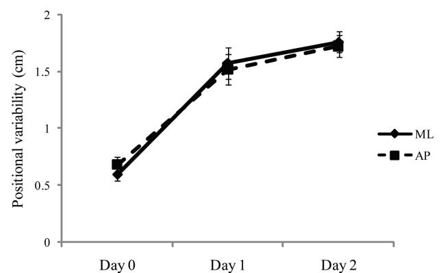
Figure 5. Experiment 2: Mean positional variability of the COP for the AP and ML axes, as a function of days. The figure illustrates the statistically significant interaction between axes and days. The error bars represent standard error of the mean. doi:10.1371/journal.pone.0066949.g005
