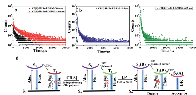
Fig. 4 Time-resolved PL decay curves of (a) HABr/CB[8]/LP/RhB and HABr/CB[8]/LP/SR101 at 500 nm, (b) HABr/CB[8]/LP/RhB at 585 nm and (c) HABr/CB[8]/LP/SR101 at 612 nm in aqueous solution at 298 K. ([HABr] = 0.1 mM, [CB[8]] = 0.05 mM, LP = 0.02 wt%, [RhB] = 4.0 \times 10^{-6} M, [SR101] = 1.3 \times 10^{-6} M, \lambda_{ex} = 300 nm, 298 K). (d) A possible diagram of the mechanism of the RTP energy transfer process for the HABr/CB[8]/LP/RhB and HABr/CB[8]/LP/SR101 systems (abs. = absorption, fluo. = fluorescence, non. rad. = non-radiation, ISC = intersystem crossing, phos. = phosphorescence, PET = phosphorescence energy transfer, DF. = delayed fluorescence).
