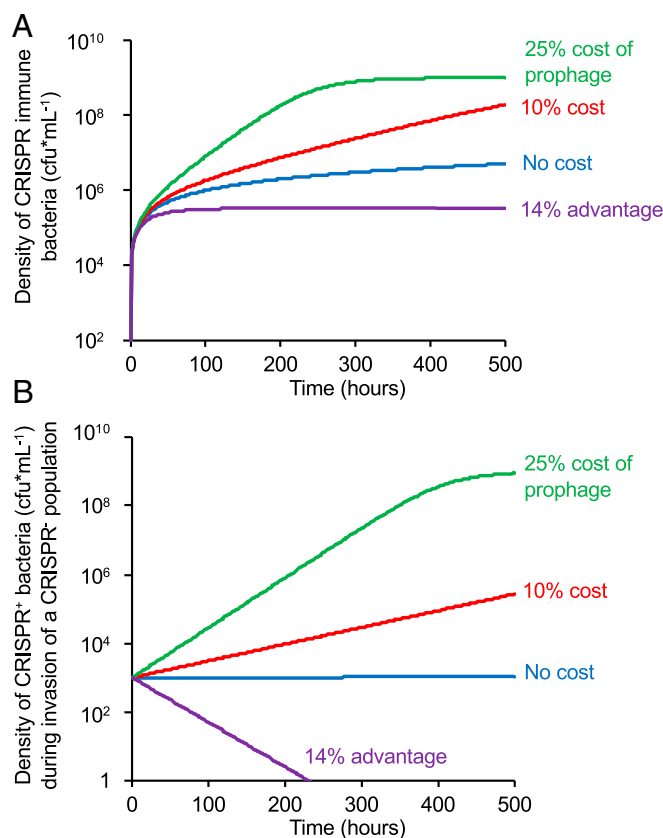
Fig. 2. Selection mediated by temperate phage. (A) The establishment of CRISPR immunity in a population of CRISPR + bacteria at equilibrium with a temperate phage. Changes in the density of CRISPR-Cas immune bacteria are depicted [colony forming units per milliliter (cfu*ml -1 )]. (B) The invasion of CRISPR + bacteria into a population of CRISPR - bacteria at equilibrium with a temperate phage. Changes in the densities of CRISPR + bacteria are depicted. Carrying the prophage is associated with a 14% advantage, a 10% cost, a 25% cost, or no cost, as indicated. The parameter values are SI Appendix, Fig. S5 C and F .
