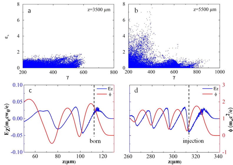
Figure 5. (a,b) are the (\epsilon_{\perp}, \gamma) space of the accelerated electrons at different laser propagation distances in nitrogen, corresponding to z = 3500 \mu\text{m} and 5500 \mu\text{m} . (c and d) show snapshots of the longitudinal wakefield potential (red line) and strength (blue line) at the time when the test electron is born and injected, where the black dashed lines in the two plots mark the electron birth and injection positions, respectively.
