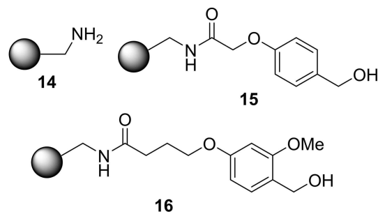
Figure 8. Structures of the ChemMatrix based resins. As commonly accepted, the sphere represents the cross-linked PEG.
