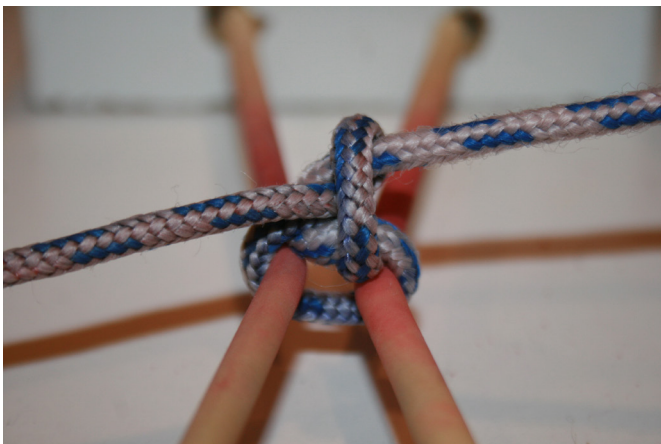
Figure 12 Initial effect of pulling on one end of reef knot causing initial loosening.
