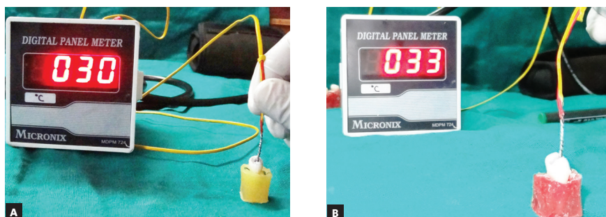
Figure 3 - Temperature measured on digital thermometer connected to J-type thermocouple: A) before stripping ; B) after stripping.
