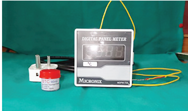
Figure 1 - J-type thermocouple connected to digital thermometer and silicon heat transfer material.
