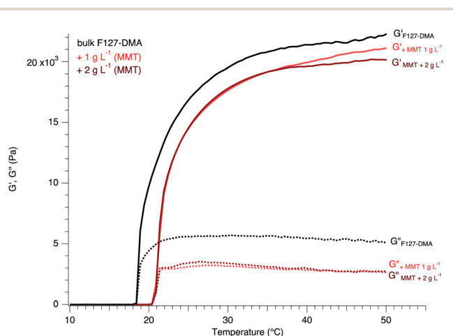
Fig. 3 Changes in both the storage ( G' , solid line) and loss ( G'' , dashed line) moduli as a function of temperature for Pluronic F127-H 2 O at a concentration of 25 wt% with PEO chains functionalized by dimethacrylate (DMA) at a rate of 88% (black) and reinforced by or including dispersions of MMT at concentrations of 1 g L -1 (red) and 2 g L -1 (dark red).
