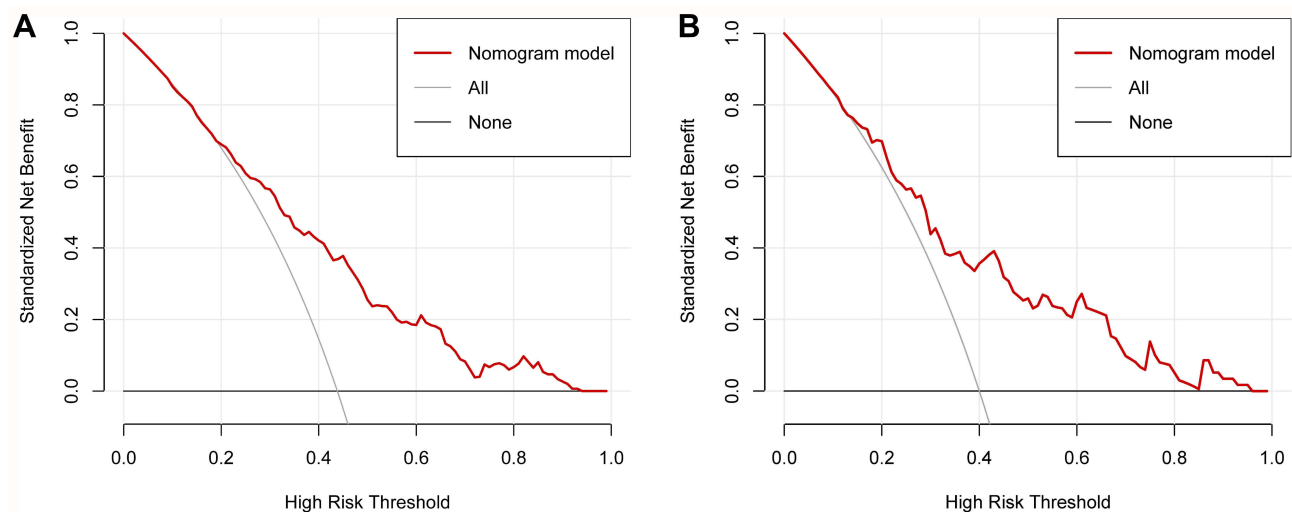
Figure 6 Decision curve analysis for the training set (A) and the validation set (B). A horizontal line indicates that all samples are negative and not treated, with a net benefit of zero. An oblique line indicates that all samples are positive. The net benefit has a negative slope.
